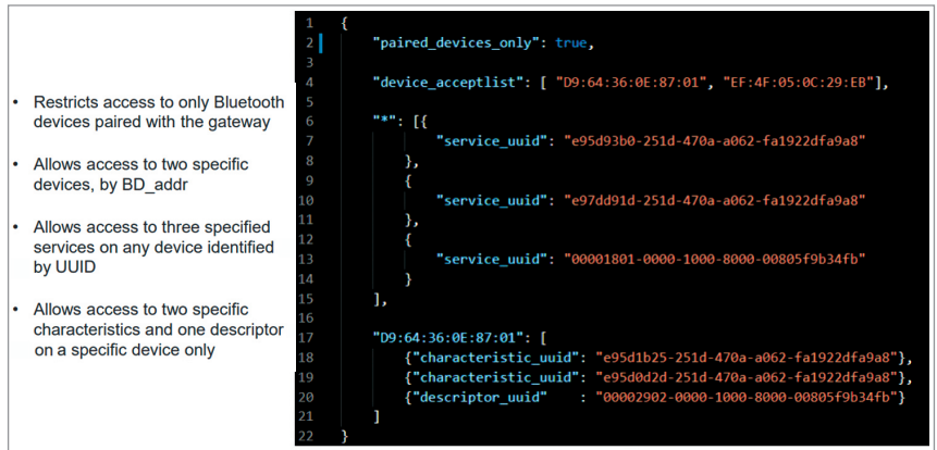
Fig. 14: Bluetooth firewall configuration
